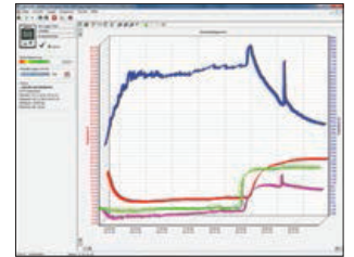
Software
